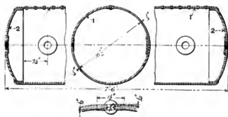
Figs. 2631-2633. Main Reservoir, Atlantic (4-4-2) Locomotive, Pennsylvania Railroad.
